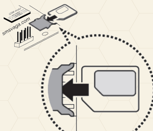
Picture 3. Inserting the micro SIM card into the electronic circuit board
