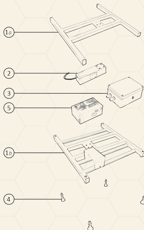
Picture 2. Main parts of the SMS Scale
